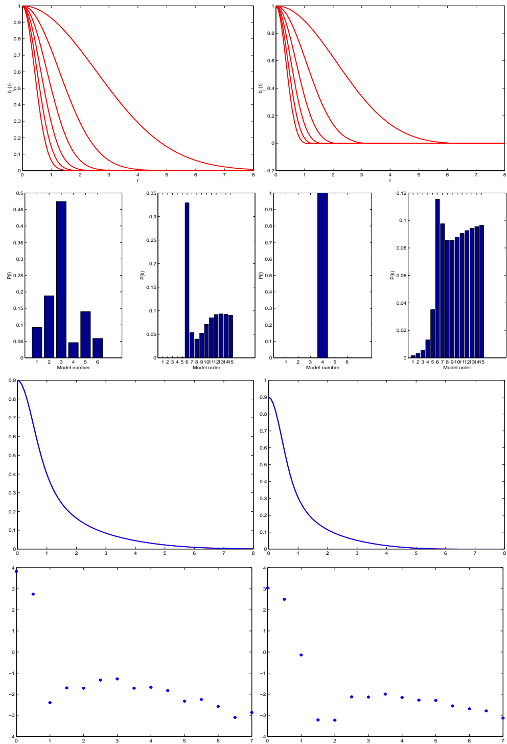
Fig. 4: Left: l = 3 Right: l = 4 a) basis functions b_j(r) , b) p(k|\mathbf{y}) and p(k|\mathbf{y}, \hat{l}) , c) \rho(r) and \hat{\rho}(r) , d) F(q_i) and \hat{F}(q_i) .
